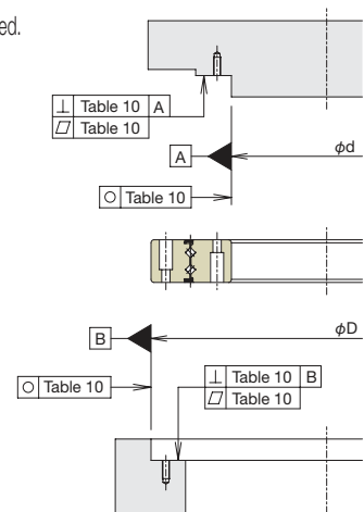
Machining accuracy of peripheral part
